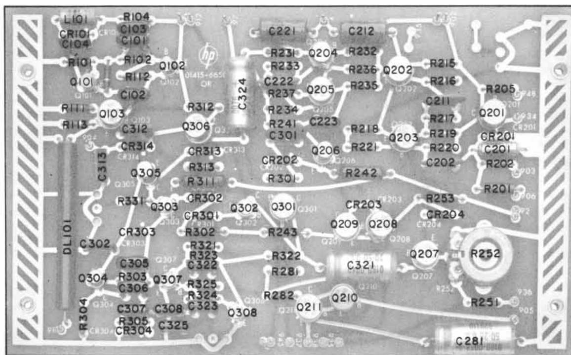
Figure IIA-2. Time Base Board A1
