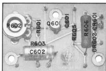
Figure IIA-6. Power Supply Board A6
