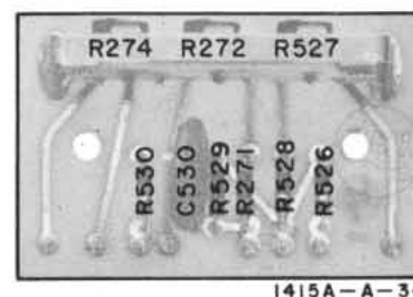
Figure IIA-5. Trimmer Board A7
