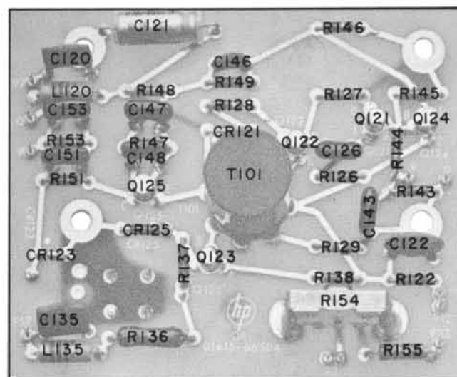
Figure IIA-8. Pulse Generator Board A2
