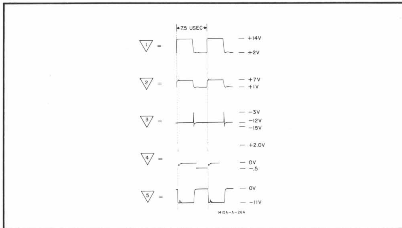
Figure 5-5. Waveforms at Test Points in Step Generator Circuit
