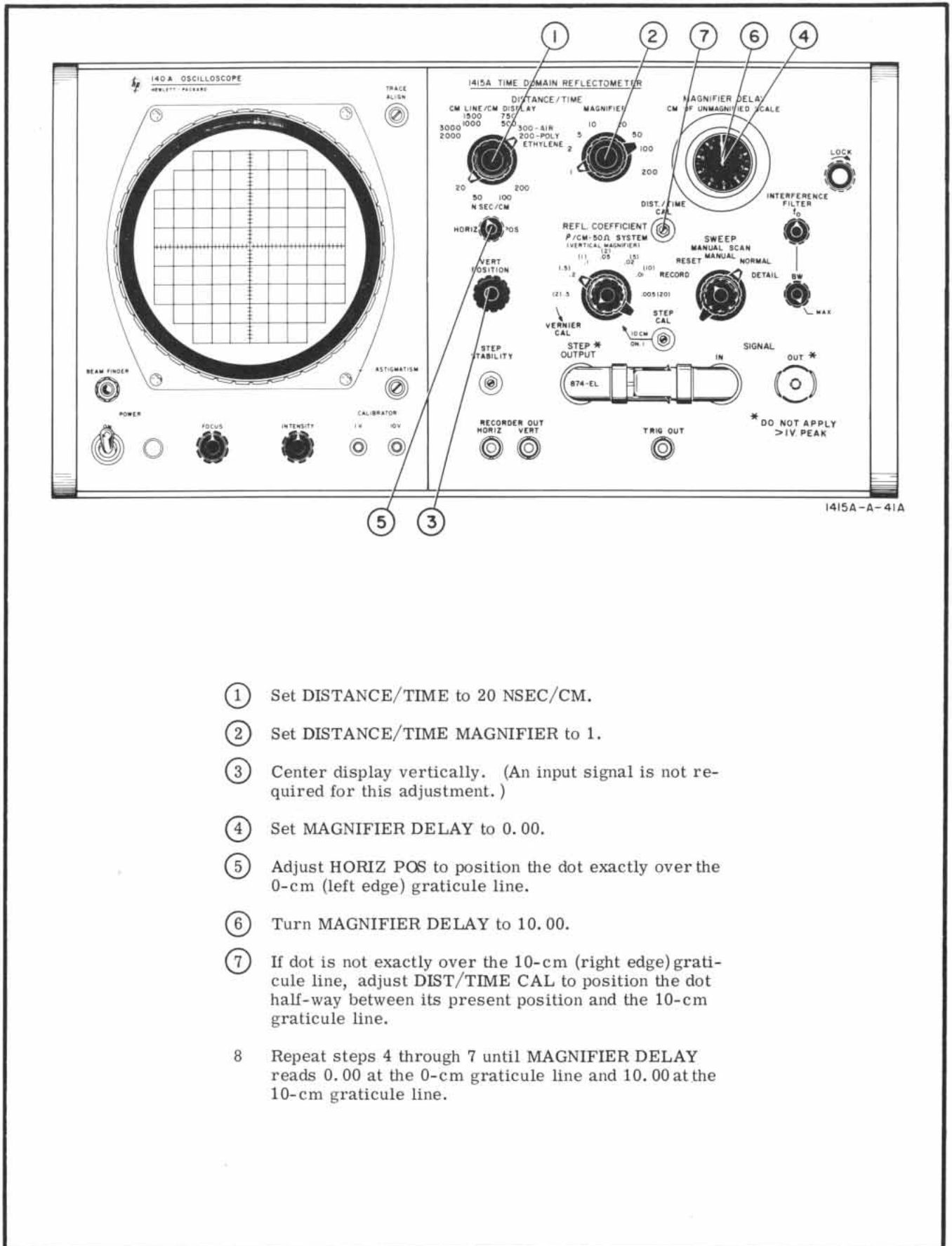
Figure 3-4. Horizontal Calibration
