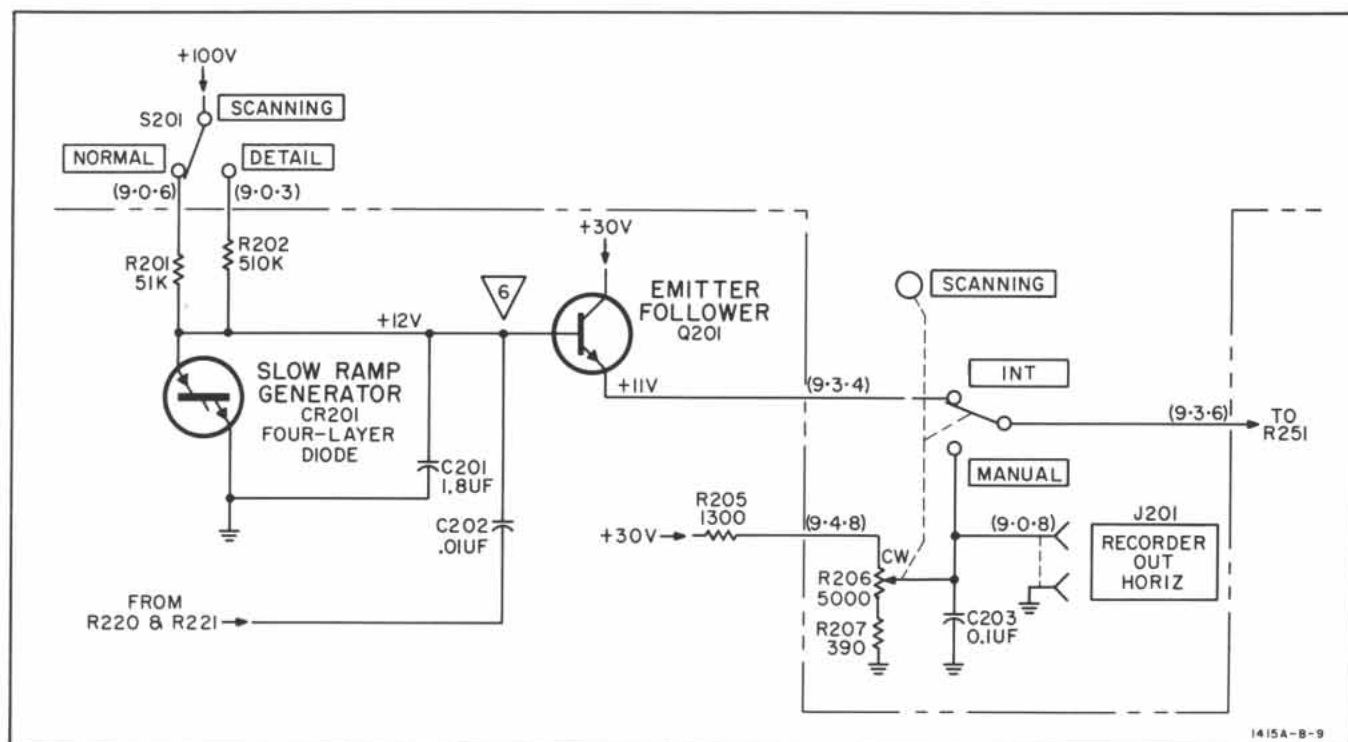
Figure IIA-3. Partial Schematic, Slow Ramp and Dot Comparator
